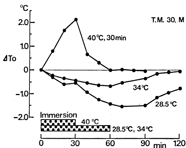
Fig. 1. Changes in oral temperature ( \Delta T_o ) due to head-out water immersion (28.5, 34 and 40°C). Oral temperature decreased 1.5°C during 28.5°C water immersion and remained low for following 60 min. In 34°C slight decrease in oral temperature was observed. During 40°C water immersion steep rise of 2.1°C in oral temperature observed at 30 min.
