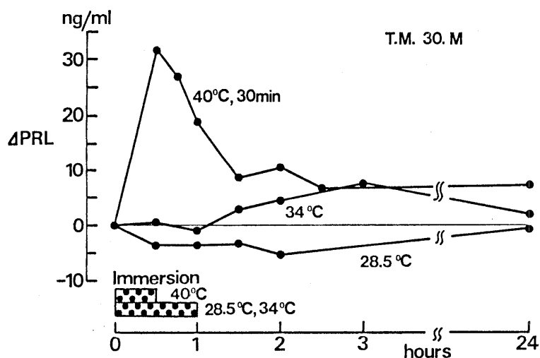
Fig. 2. Changes in serum prolactin ( \Delta PRL ) level due to head-out water immersion (28.5, 34 and 40°C). Serum prolactin decreased 48% during 28.5°C water immersion. In 34°C serum prolactin level kept constant and slightly increased after cessation of water immersion. Marked increase (578%) in serum prolactin was observed during 40°C water immersion. In every experiment serum prolactin level returned to control level after 24 hours.
