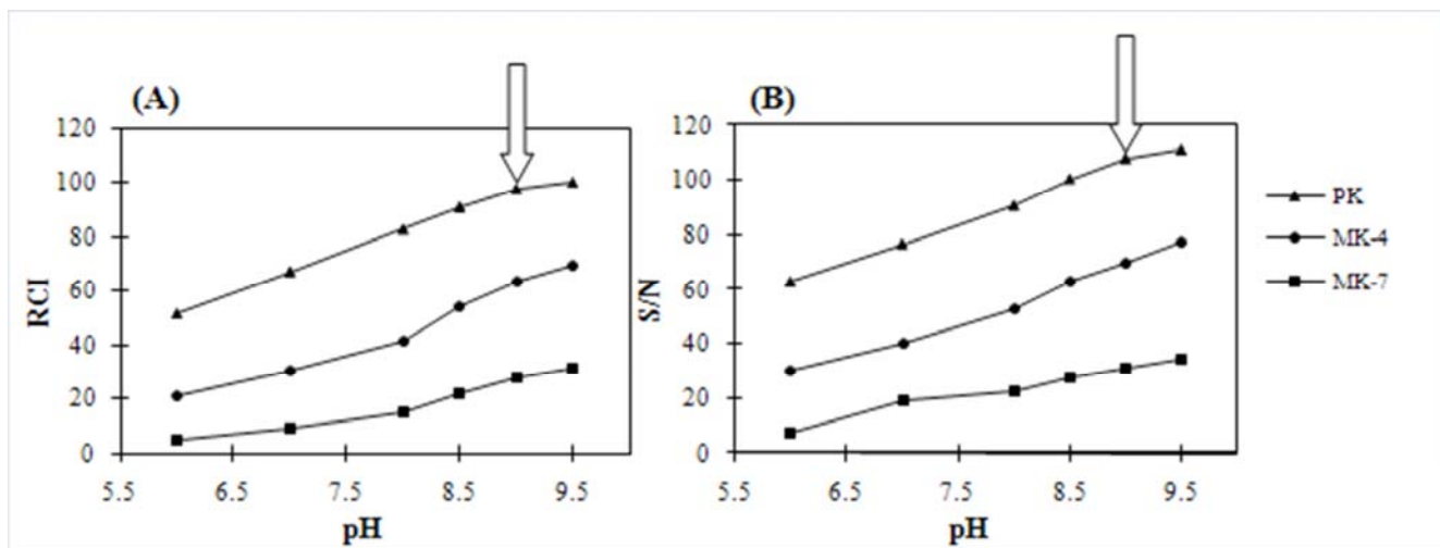
Fig. 2 . Effects of pH of imidazole-HNO 3 buffer on (A) CL intensity and (B) S/N ratio. Sample concentration was 0.5 μg mL -1 for each vitamin K.
