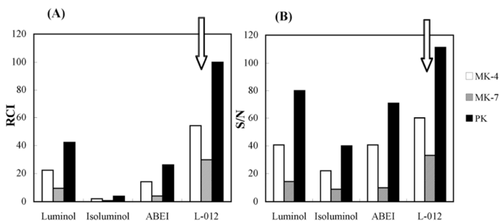
Fig. 3. Effects of different luminol derivatives on (A) CL intensity and (B) S/N ratio. Samples concentrations were 0.5 μg mL -1 from each vitamin K.
