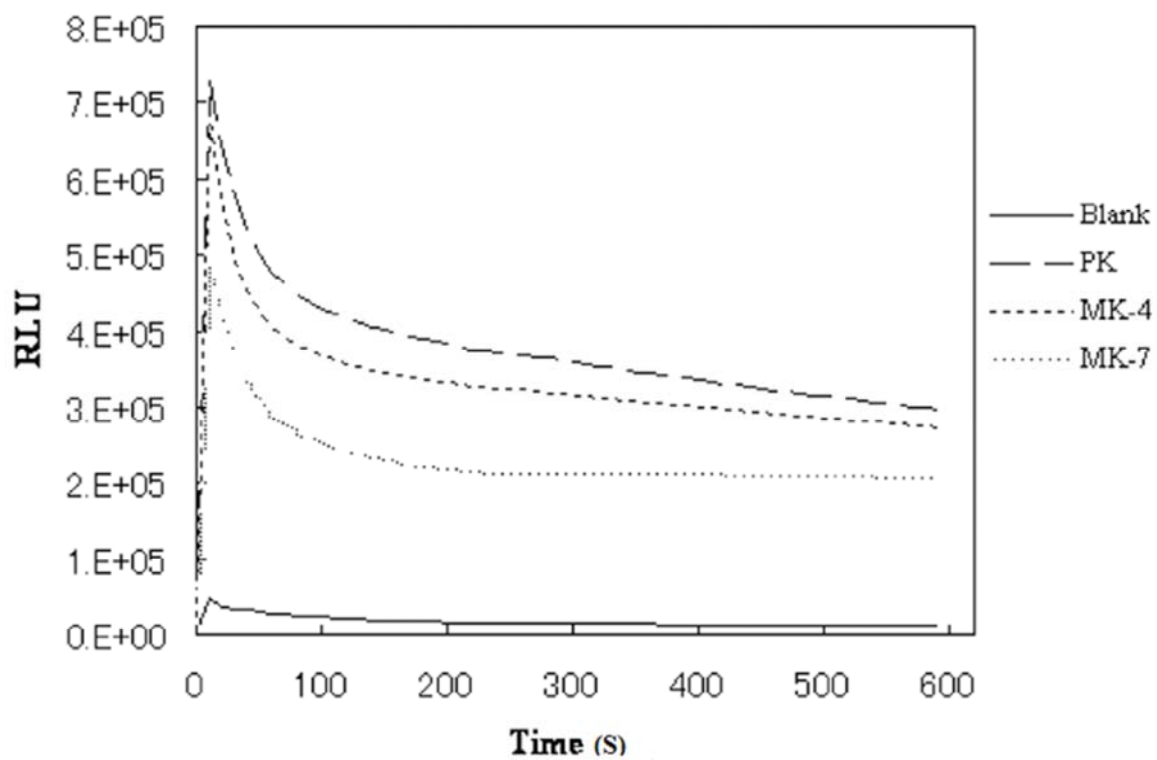
Fig. 1. Time profiles of CL emission obtained by UV irradiation products from vitamin K homologues with 3 \mu\text{mole L}^{-1} of L-012.
