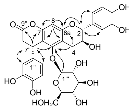
Figure 4. Selected HMBC correlations (H to C) of 2
