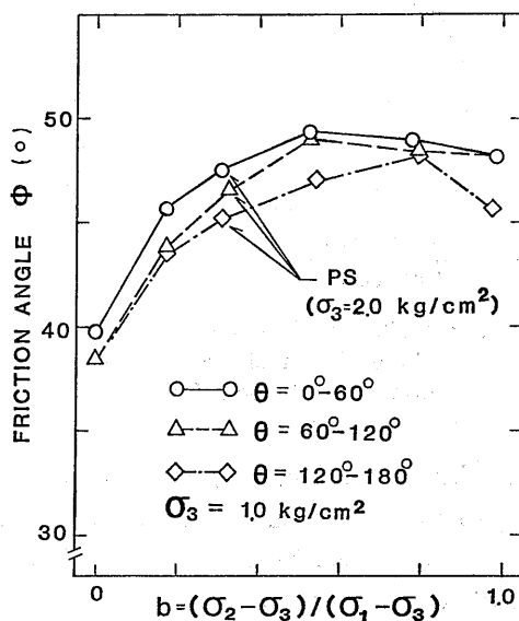
Fig. 5 Failure surface shown in \phi - b diagram for cubical triaxial and plane strain tests on a sand with cross-anisotropic fabric
