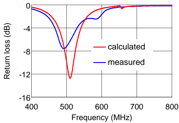
Figure 5 Return loss characteristics of antenna F-3.
