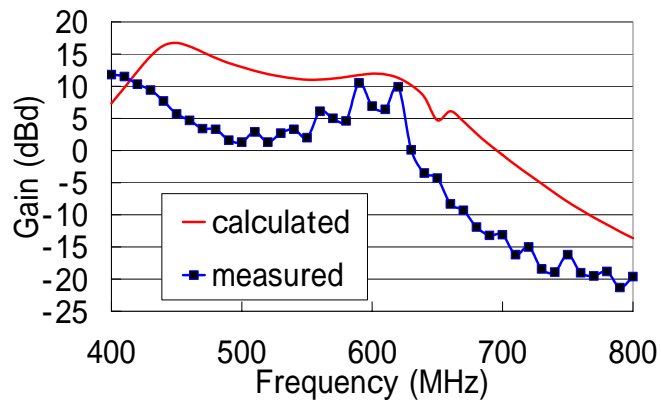
Figure 6 Actual gain of antenna F-3 in x direction.
