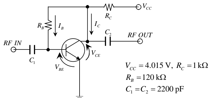
Figure 2 Amplifier circuit.
