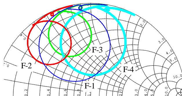
Figure 3 Calculated input impedance characteristics.
