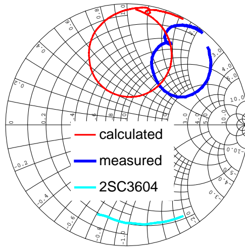
Figure 4 Input impedance of antenna F-3 and S_{11} parameter of amplifier circuit.
