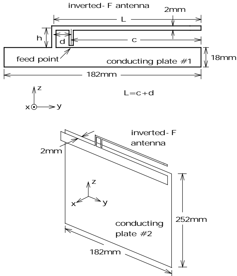
Figure 1 Inverted-F antenna mounted on side of small conducting plate.
