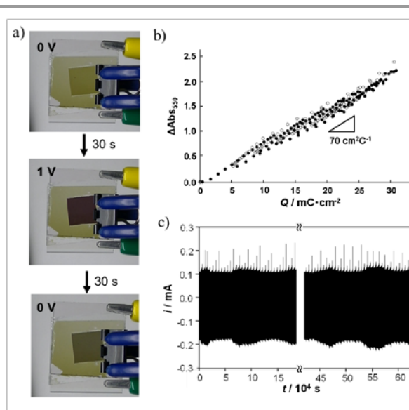
Fig. 3 a) Colour changes of the electrochromic cell. b) Dependence of \Delta\text{Abs}_{550} on Q from 0 to 500 s. The filled ( \bullet ) and open ( \circ ) circles indicate charging at 1.0 V and discharging at 0.0 V, respectively. c) Durability of the electrochromic cell (10000 cycles) during applied potential step ( E_{\text{appl}} = 0.0 and 1.0 V) cycles every 30 s.
