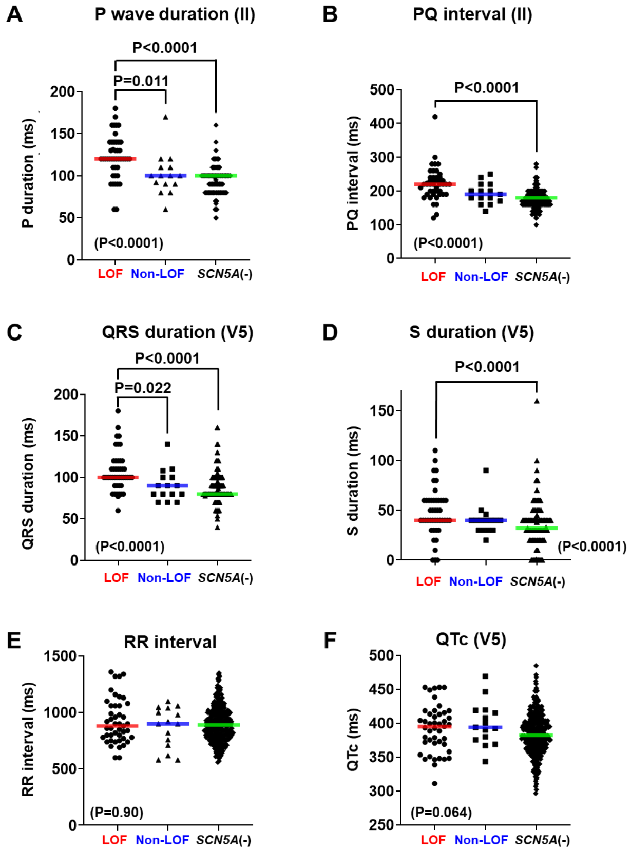
Supplemental Figure S2. ECG parameters of patients with BrS of three subgroups classified by the Na channel function properties. A. P wave duration, B. PQ interval, C. QRS duration, D. S duration, E. RR-interval, and F. Corrected QT interval by Bazett's formula (QTc) of three groups are shown. Patients carrying the LOF- SCN5A mutations exhibited significantly impaired ECG conduction parameters compared with those with Non-LOF and/or SCN5A mutation non-carriers ( SCN5A (-)). The horizontal bar represents the median. Statistical analysis was performed using Kruskal-Wallis test and post-hoc Dunn's test for multiple comparisons. P values with parentheses indicate statistical significance among three groups.
