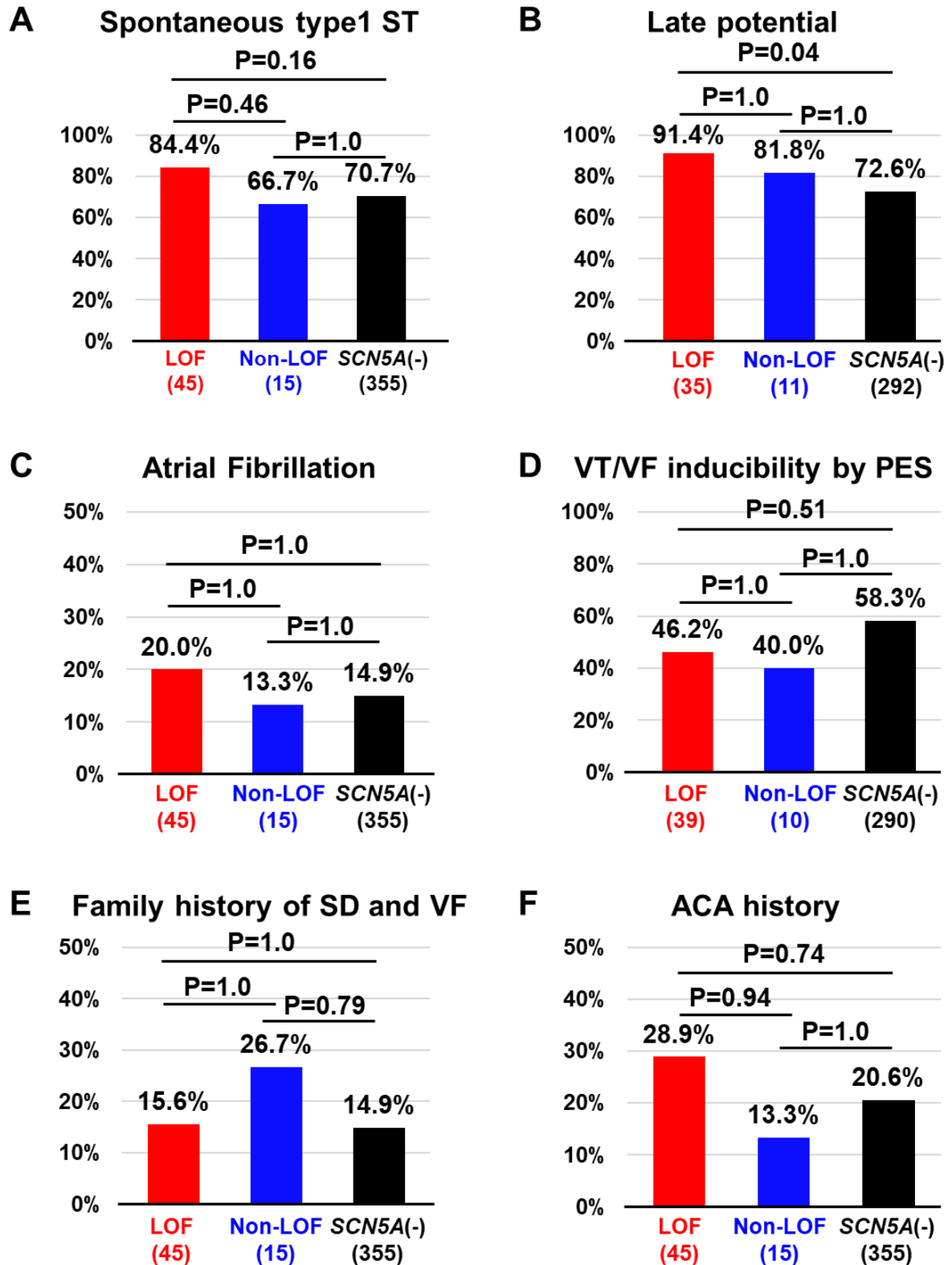
Supplemental Figure S3. Electrophysiological and clinical findings among three groups of BrS cohort-I.
