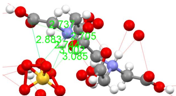
図 5 EDTA·H 2 SO 4 ·H 2 O の分子内水素結合 ( d_{N-O} = 2.705 \text{ \AA} , 2.737 \text{ \AA} ) と分子間水素結合 ( d_{N-O} = 2.744 \text{ \AA} , 3.002 \text{ \AA} , d_{O-O} = 2.883 \text{ \AA} , 3.085 \text{ \AA} ) (Shkol'nikova et al. 1993) [9].
