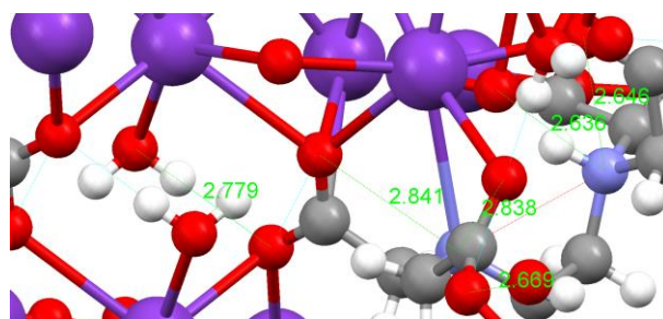
図 23 [\text{K}_3(\text{EDTA-3H})]\cdot 2\text{H}_2\text{O} の分子内水素結合 ( d_{\text{N-O}} = 2.636 \text{ \AA}, 2.646 \text{ \AA}, 2.838 \text{ \AA}, 2.841 \text{ \AA} ) と分子間水素結合 ( d_{\text{N-O}} = 2.838 \text{ \AA}, 2.841 \text{ \AA}, d_{\text{O-O}} = 2.669 \text{ \AA}, 2.779 \text{ \AA} ) (Krawczyk & Lis 2011) [17].
