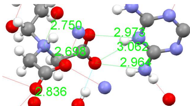
図 20 (\text{HC}_3\text{N}_3(\text{NH}_2)_2)_2[\text{EDTA-2H}]\cdot 2\text{H}_2\text{O} の分子内水素結合 ( d_{\text{N-O}} = 2.698 \text{ \AA}, 2.737 \text{ \AA} ) と分子間水素結合 ( d_{\text{N-O}} = 2.750 \text{ \AA}, 2.964 \text{ \AA}, 2.973 \text{ \AA}, 3.062 \text{ \AA}, d_{\text{O-O}} = 2.836 \text{ \AA} ) (Vella-Zarb et al. 2014) [27].
