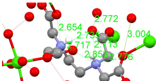
図 19 \text{Ca}[\text{EDTA-2H}]\cdot 2\text{H}_2\text{O} の分子内水素結合 ( d_{\text{N-O}} = 2.654 \text{ \AA}, 2.713 \text{ \AA}, 2.717 \text{ \AA}, 2.735 \text{ \AA}, 2.776 \text{ \AA}, 2.853 \text{ \AA} ) と分子間水素結合 ( d_{\text{O-O}} = 2.772 \text{ \AA}, 3.004 \text{ \AA} ) (Zabel et al. 2009) [26].
