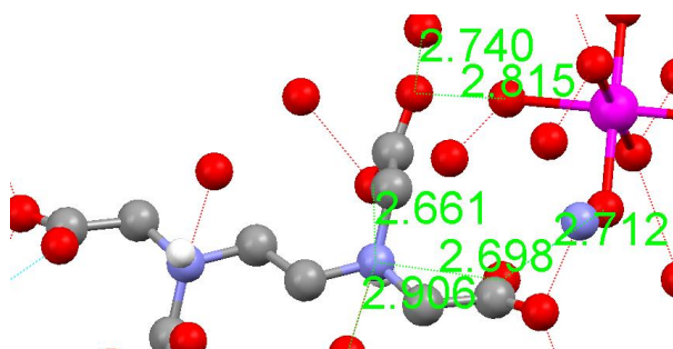
図 17 [\text{Mn}(\text{H}_2\text{O})_6][\text{EDTA-2H}] の分子内水素結合 ( d_{\text{N-O}} = 2.661 \text{ \AA}, 2.698 \text{ \AA} ) と分子間水素結合 ( d_{\text{N-O}} = 2.906 \text{ \AA}, d_{\text{O-O}} = 2.712 \text{ \AA}, 2.740 \text{ \AA}, 2.815 \text{ \AA} ) (Ma & Niu 2003) [24].
