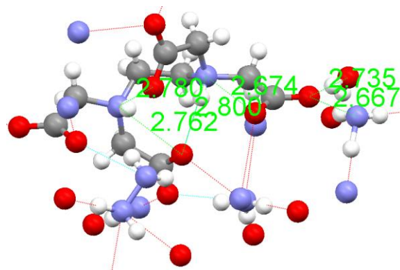
図 22 (\text{NH}_4)(\text{N}_2\text{H}_5)[\text{EDTA-2H}](\text{NH}_3)\cdot 2\text{H}_2\text{O} の分子内水素結合 ( d_{\text{N-O}} = 2.674 \text{ \AA}, 2.727 \text{ \AA}, 2.728 \text{ \AA}, 2.762 \text{ \AA}, 2.780 \text{ \AA}, 2.800 \text{ \AA} ) と分子間水素結合 ( d_{\text{N-O}} = 2.667 \text{ \AA}, d_{\text{O-O}} = 2.735 \text{ \AA} ) (Sivasankar & Sonia 2016) [29].
