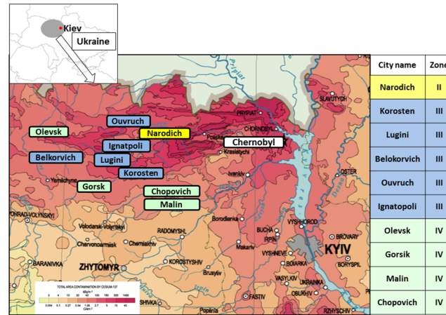
Fig 1. The study area. 10 cities were selected from north part of Zhitomir region, Ukraine, southwest from Chernobyl. In Ukraine, a classification of 4 contamination zones was established. The zones were defined according to soil contamination levels of 137 Cs as zone I (> 1480 kBq/m 2 ), zone II (555 kBq/m 2 –1480 kBq/m 2 ), zone III (185 kBq/m 2 –555 kBq/m 2 ) and zone IV (37 kBq/m 2 –185 kBq/m 2 ). The 10 cities we chosen were classified to zone II-IV as shown in the table. This map was modified from copyright free maps provided by DesignExchange Co. Ltd and Ministry of Emergency and Protection of Chernobyl-affected people, Ukraine.
