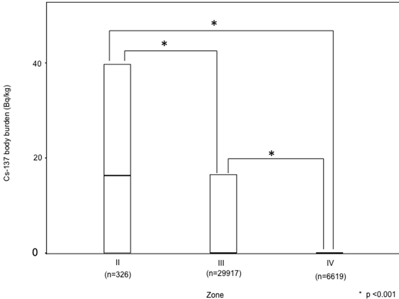
Fig 3. Cs-137 body burden in the residents living in each zone. The end of the box indicate the positions of the 75th percentiles of the data. The Cs-137 body burden was significantly higher in more contaminated zone.
