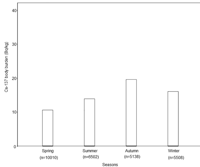
Fig 2. Seasonal difference of Cs-137 body burden in residents. The end of the box indicate the positions of the 75th percentiles of the data. The median Cs-137 body burden was below the detectable level in each season however significantly higher in autumn than other seasons ( p < 0.001 ).
