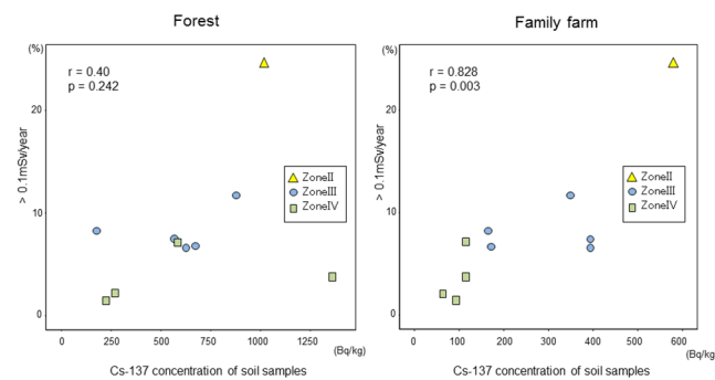
Fig 4. Correlation between mean 137 Cs concentration of soil samples and rate of population with dose >0.1 mSv/year of each city.
