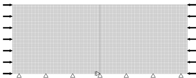
Fig.10 Mesh division
