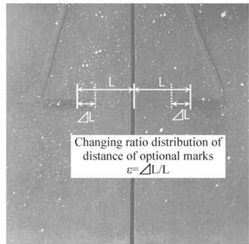
Fig.7 The image of concrete surface after cutting
