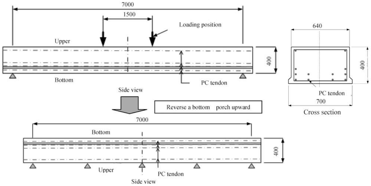
Fig.5 Pre-tension concrete beam
