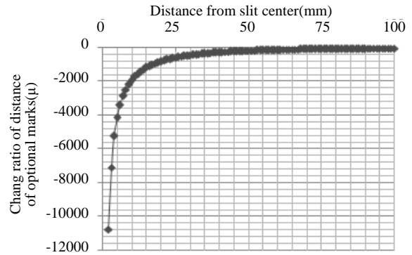
Fig.11 Changing ratio distribution of distance of optional marks (FE analysis)
