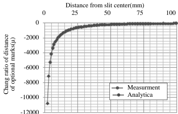
Fig.12 Changing ratio distribution of distance of optional marks
