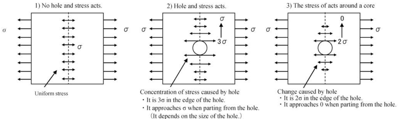
Fig.2 Change of the stress of the horizontal direction
