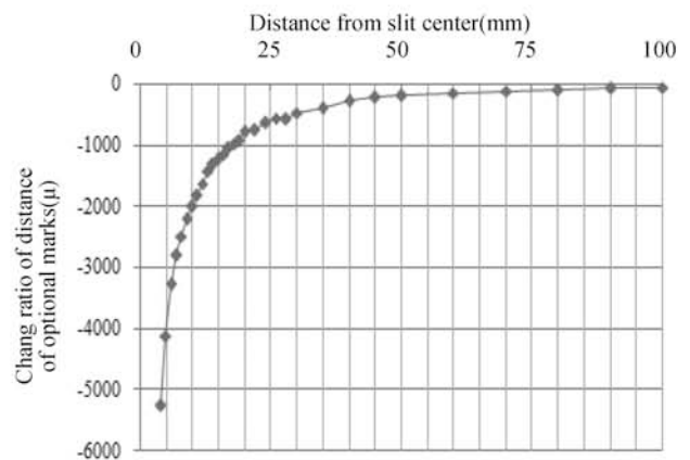
Fig.8 Changing ratio distribution of distance of optional marks
