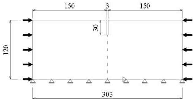
Fig.9 Analytical model
