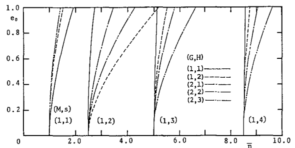
Fig. 2 Magnitude e_0 of the initial deflection vs natural frequency \bar{n} for the case of M=1 .
