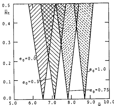
Fig. 7 Unstable regions of a square plate : \omega_1^1 + \omega_2^1 , G=2 and H=2 .
