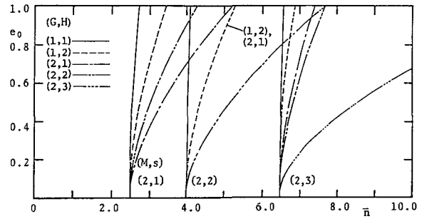
Fig. 3 Magnitude e_0 of the initial deflection vs natural frequency \bar{n} for the case of M=2 .
