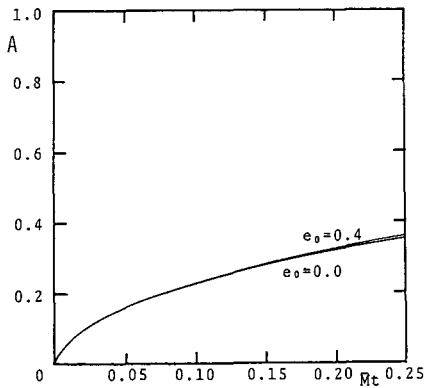
Fig. 11 Maximum amplitudes of unstable motions : \omega_1^2 + \omega_2^2 , G=1 and H=2 .
