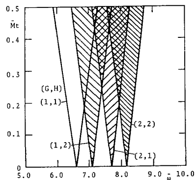
Fig. 6 Unstable regions of a square plate : \omega_1^1 + \omega_2^2 and e_0=0.5 .
